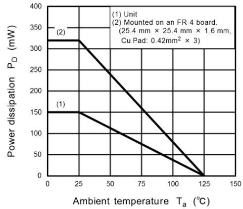
Fig. 7.4 P_D - T_a
